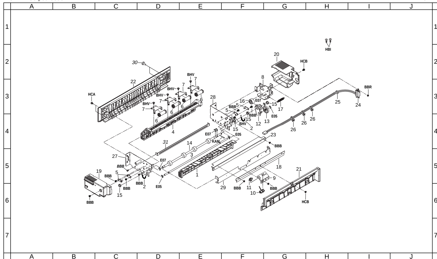
FIG. 1 Output feeder
